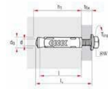
WALL ANCHOR FITTINGS
