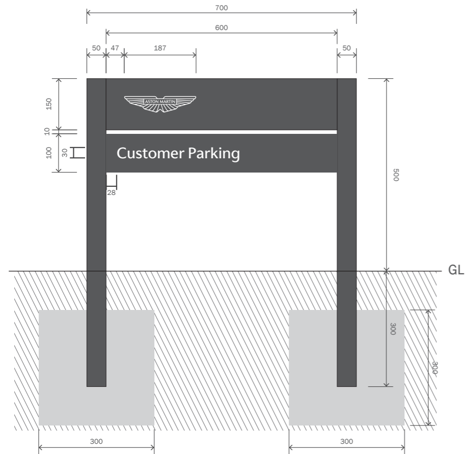
FRONT ELEVATION SCALE_1:10
