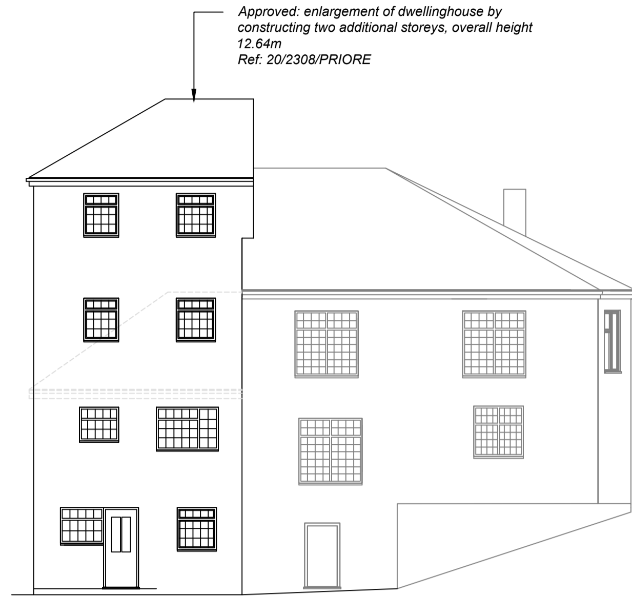
01. Proposed Front Elevation
