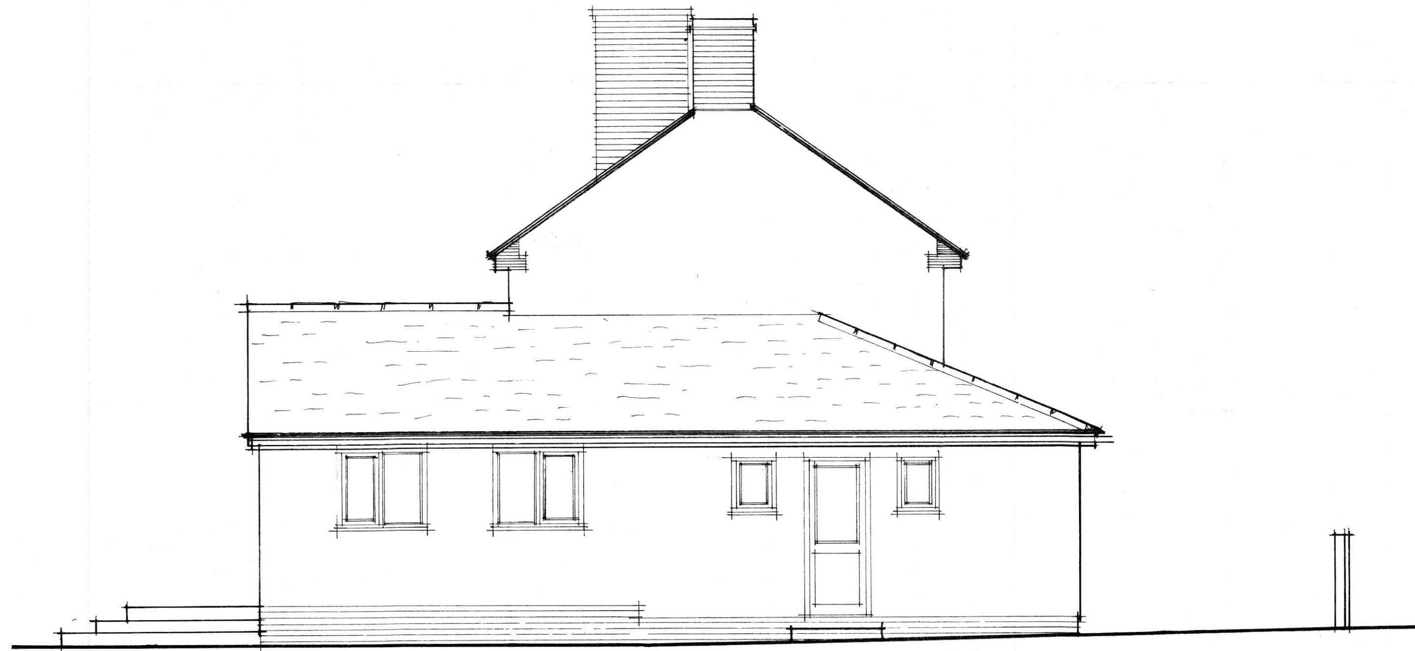
SOUTH-EAST ELEVATION
