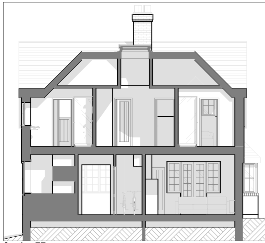
Section EE
