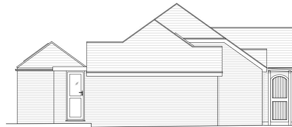
Left Side Elevation As Proposed
