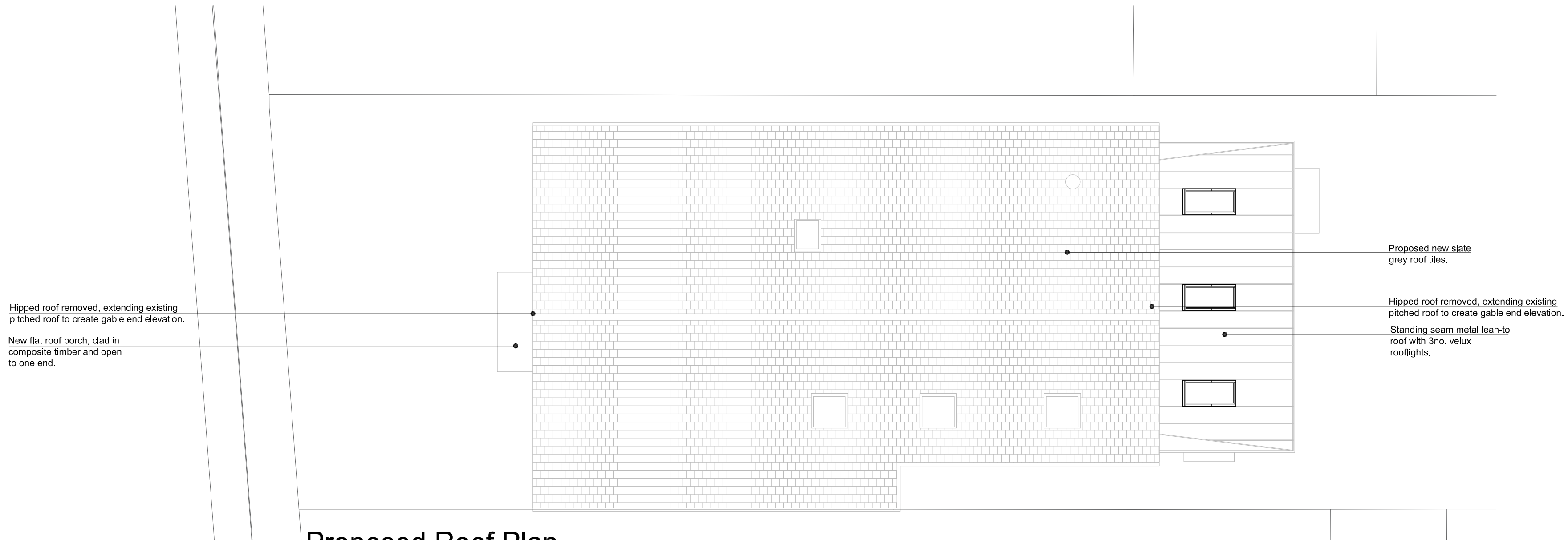
Proposed Roof Plan Scale 1:100 @ A2
