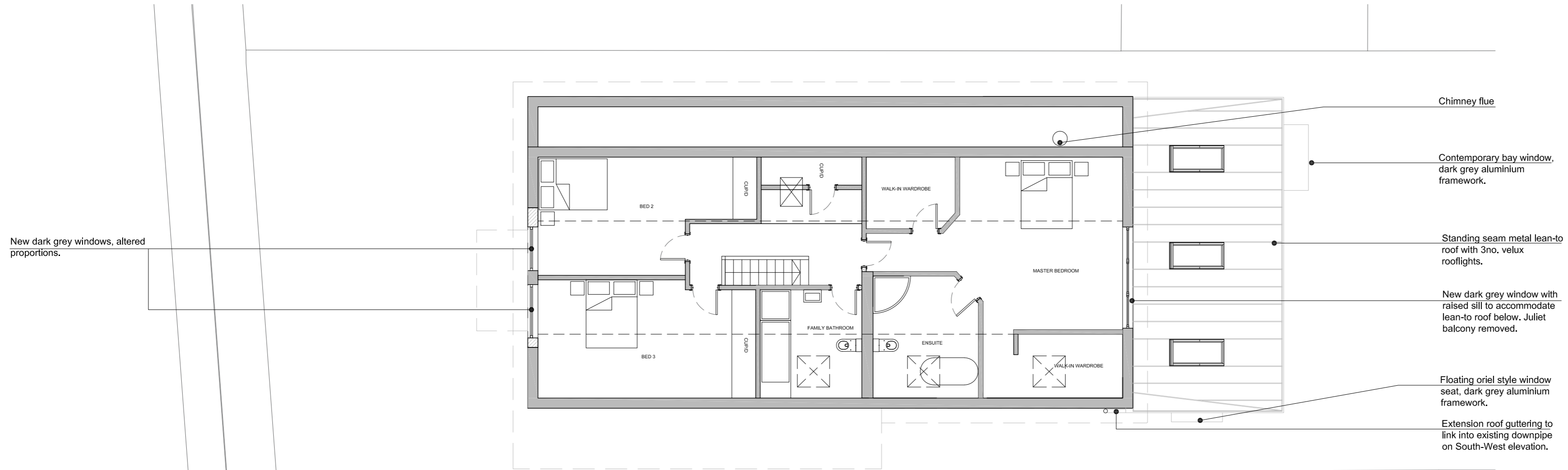
Proposed First Floor Plan Scale 1:100 @ A2
