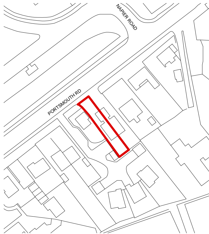
LOCATION PLAN 1:1250
