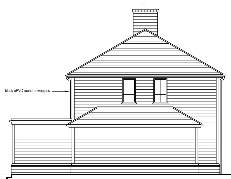
Proposed Side Elevation (South East)
