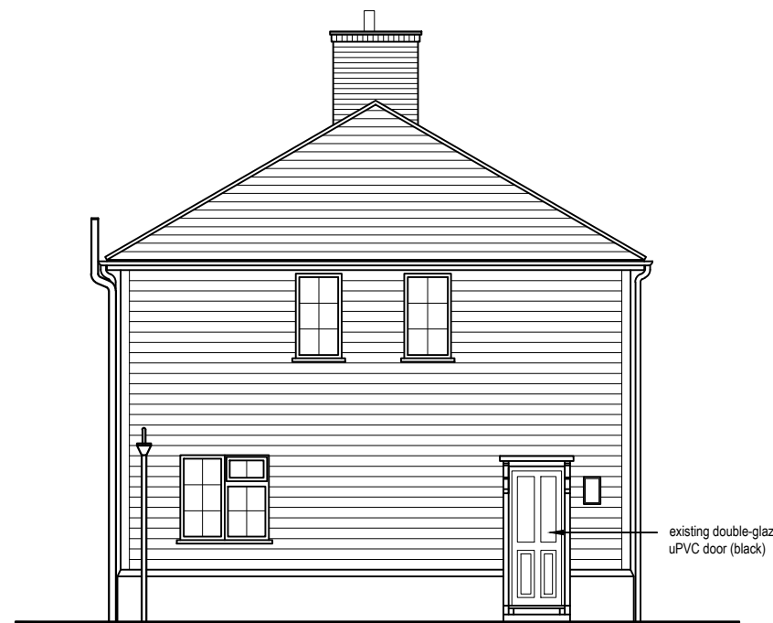
Proposed Side Elevation (South East)
