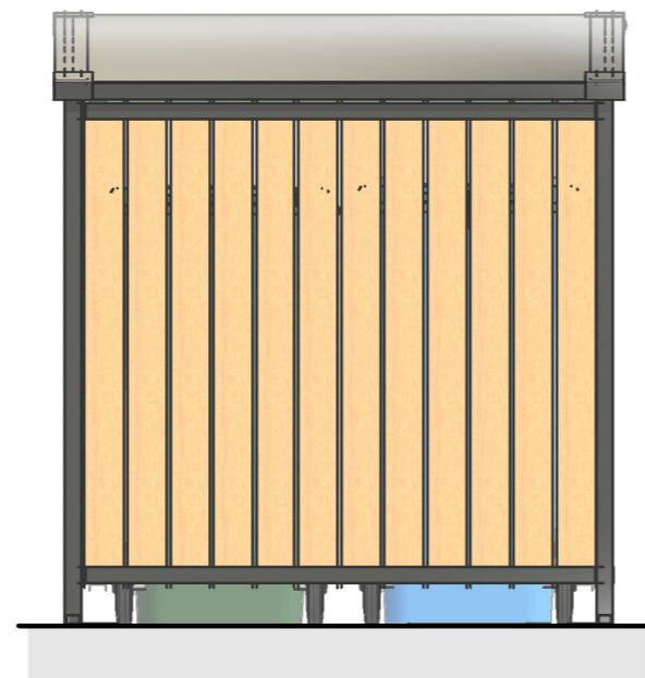
4 REAR SCALE 1 : 20
