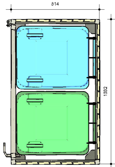
1 BIN SHED SCALE 1 : 20
