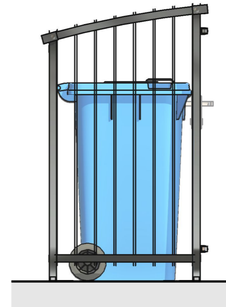
3 RIGHTSIDE SCALE 1 : 20
