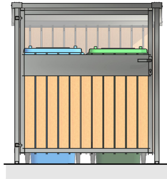
2 FRONT SCALE 1 : 20
