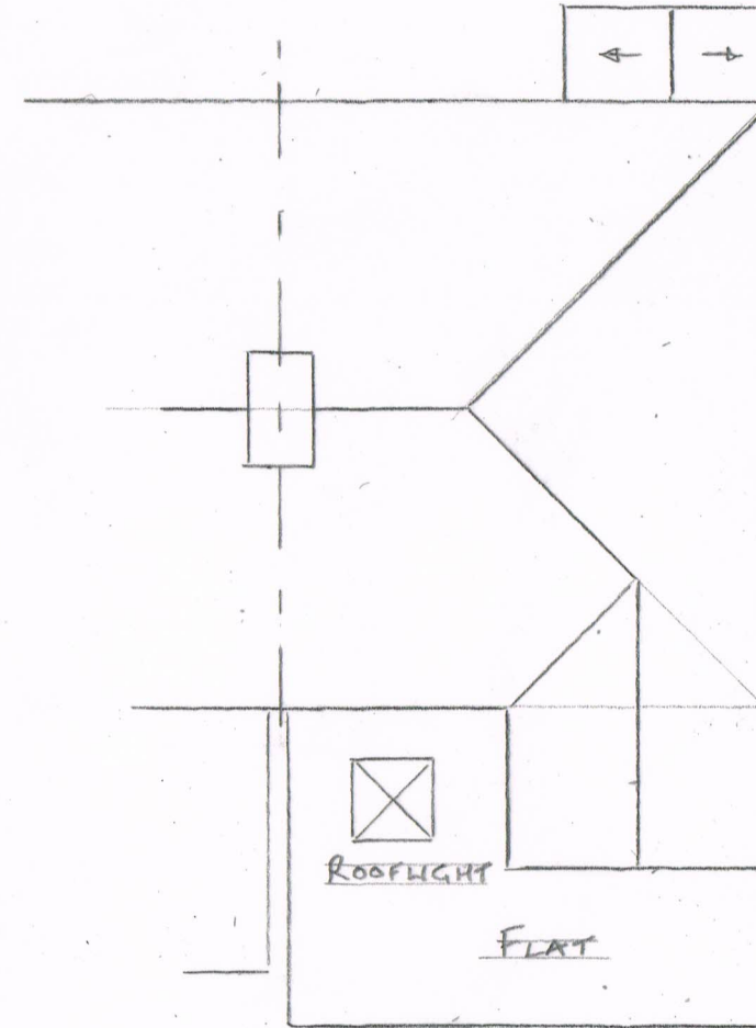
ROOF PLAN 1/100
