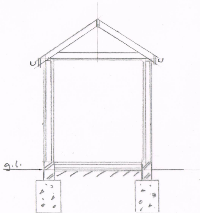
SECTION B-B 1/50
