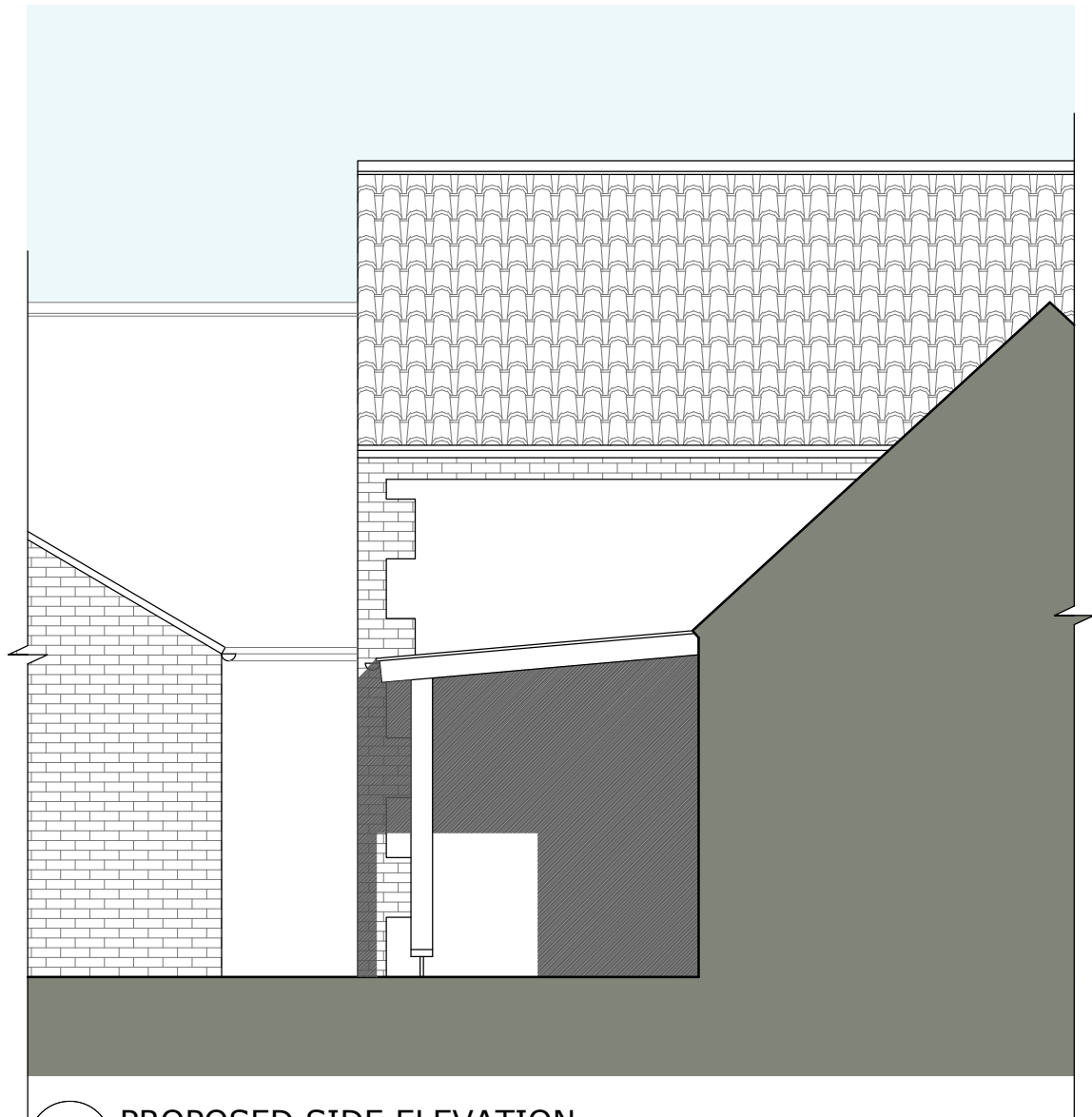
03 PROPOSED SIDE ELEVATION 1:50
