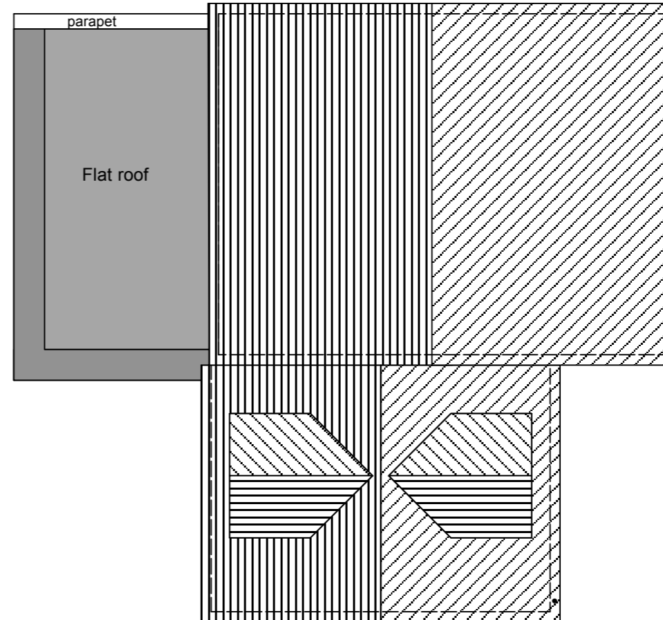
02 Proposed Roof Plan
