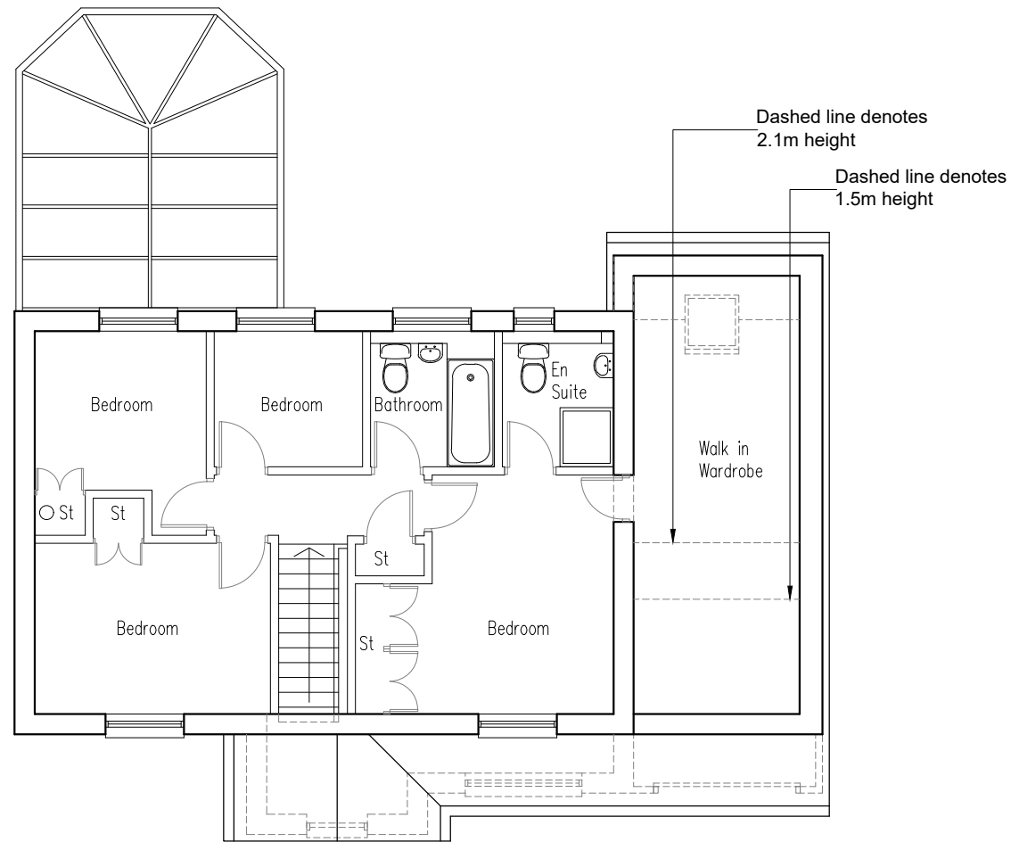
1:100 Proposed First floor plan
