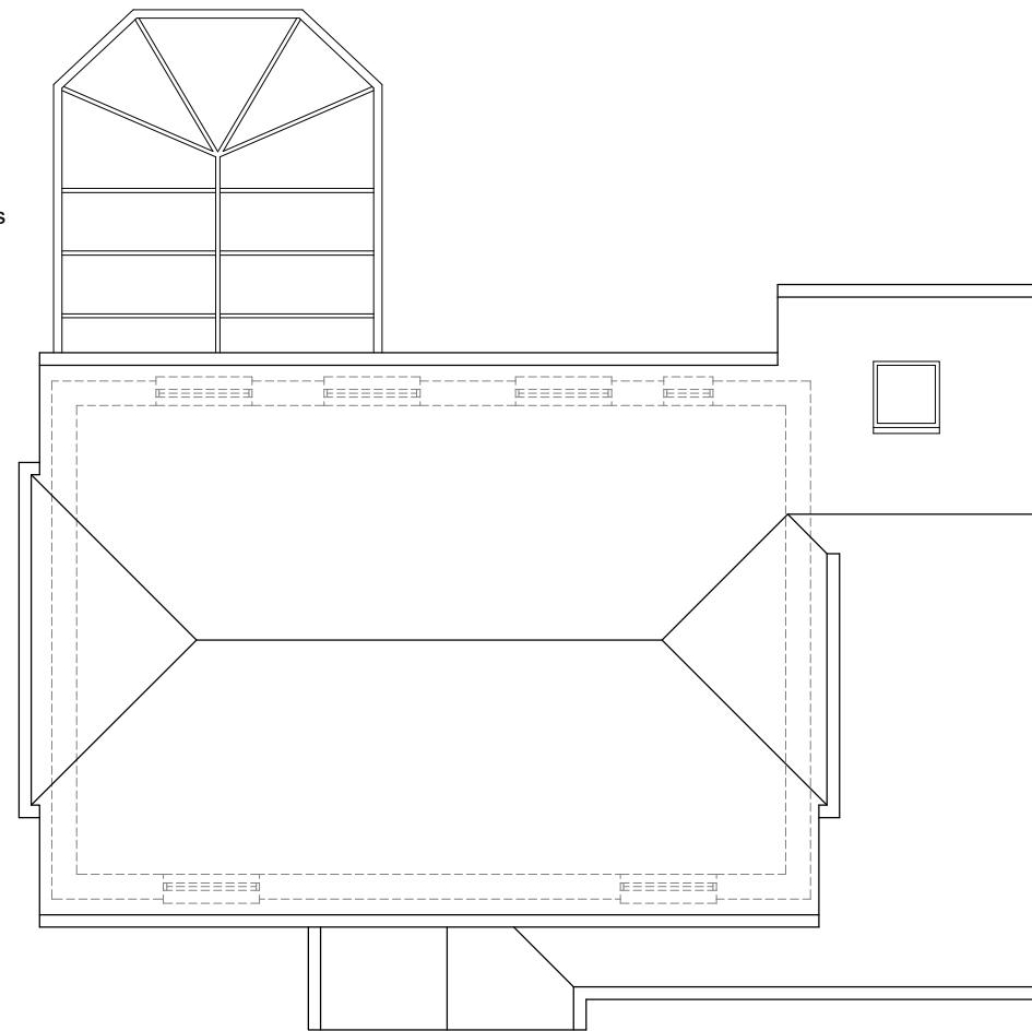
1:100 Proposed Roof plan
