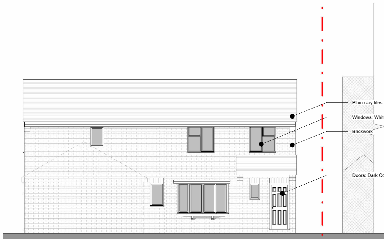
Front Elevation
