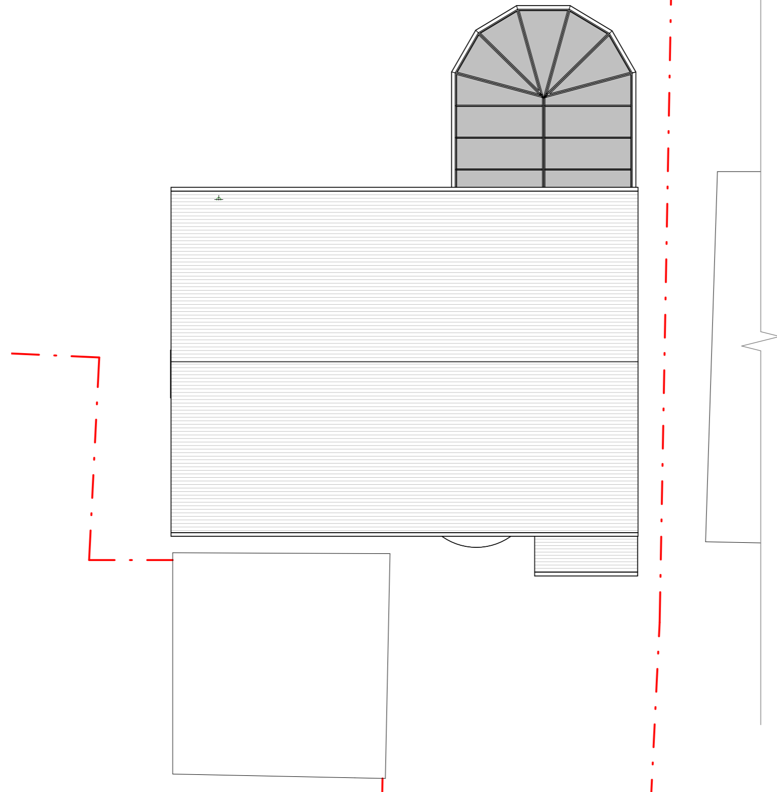
Roof Plan
