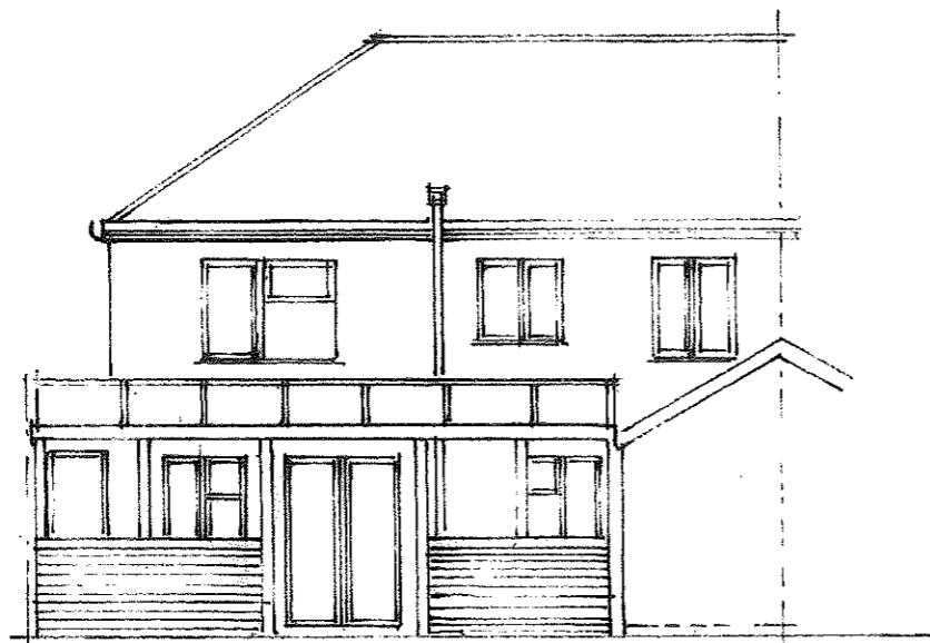
EXIST REAR ELEV. W.
