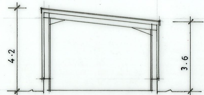
SECTION 1:100
