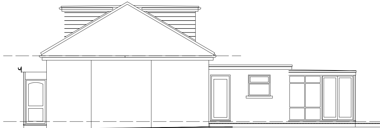
SIDE ELEVATION AS PROPOSED
