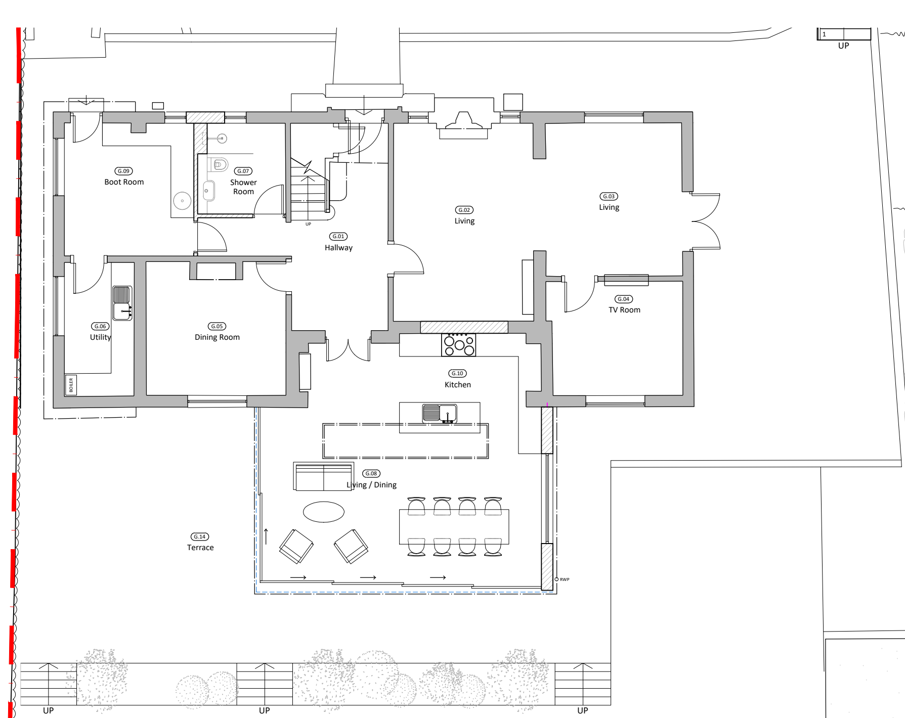
Ground Floor Plan - Main House
