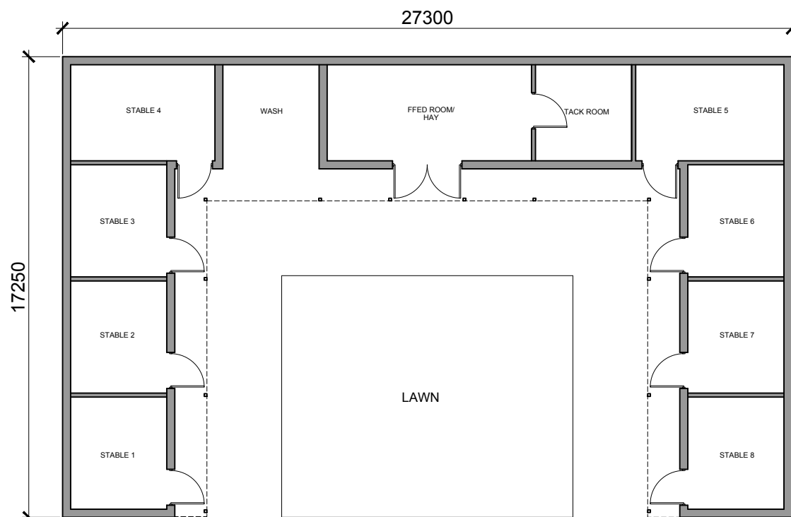
PROPOSED STABLE BLOCK FLOOR PLAN
