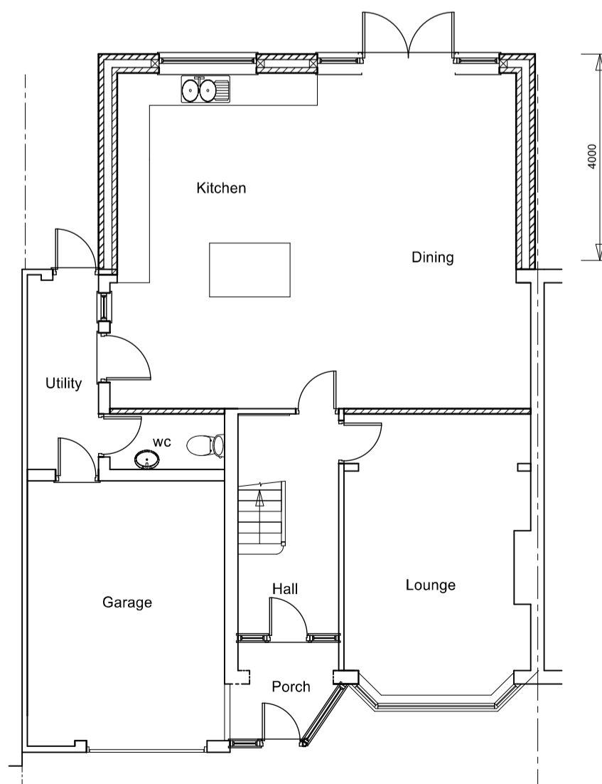
GROUND FLOOR (PROPOSED)
