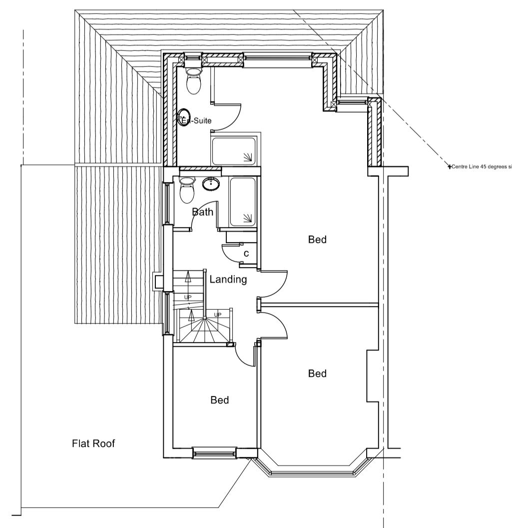
FIRST FLOOR (PROPOSED)
