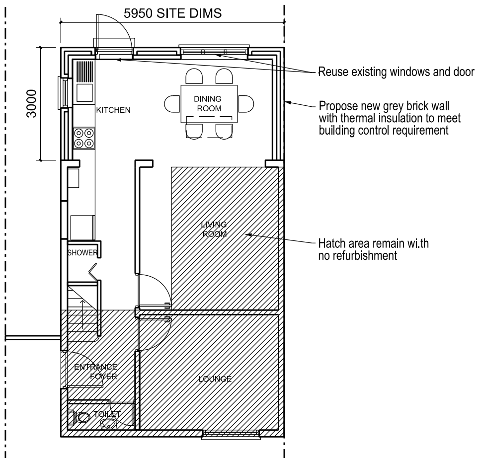
Propose Ground Floor Plan
