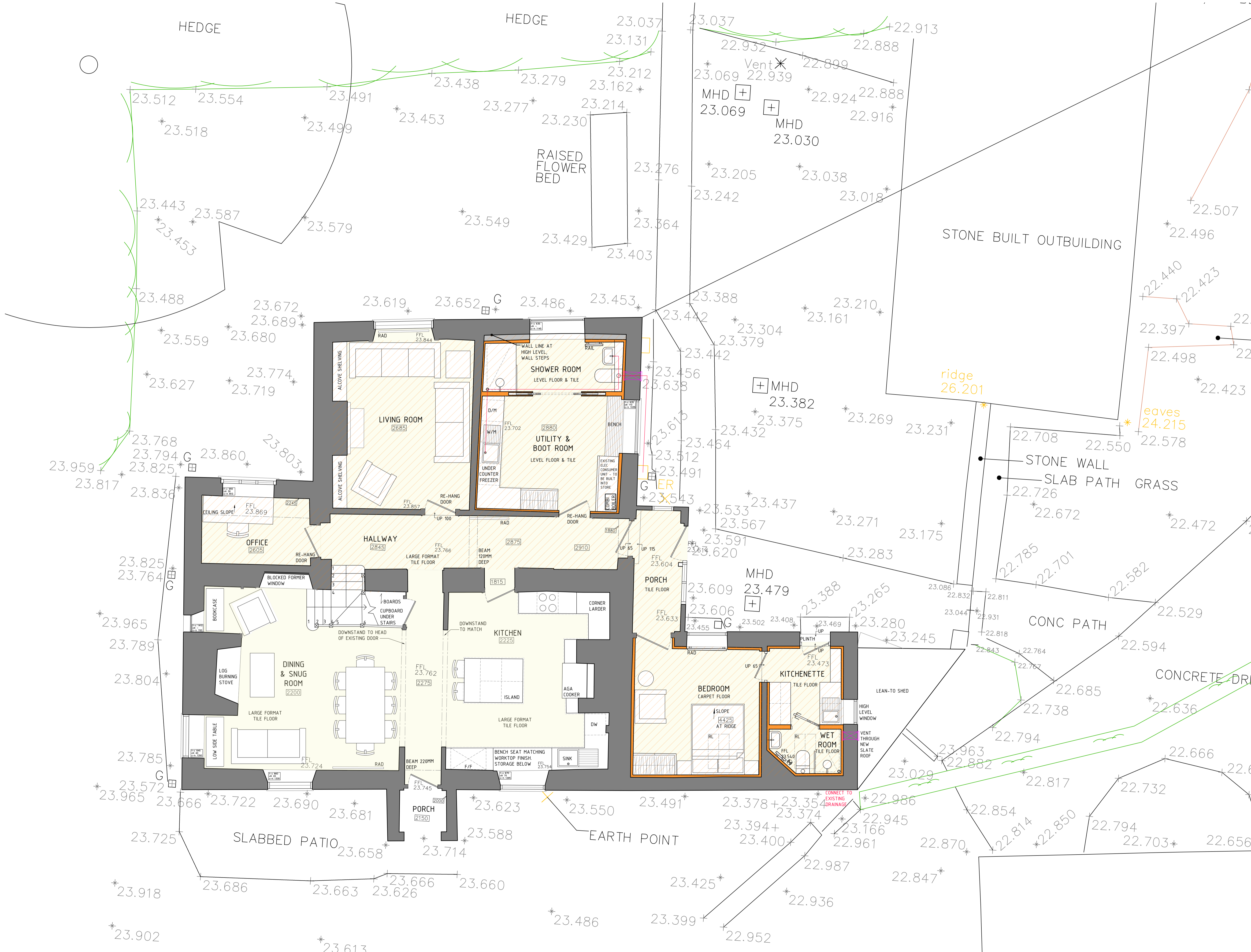
PROPOSED GROUND FLOOR PLAN - MERGED 1:100 @ A3 // 1:50 @ A1
