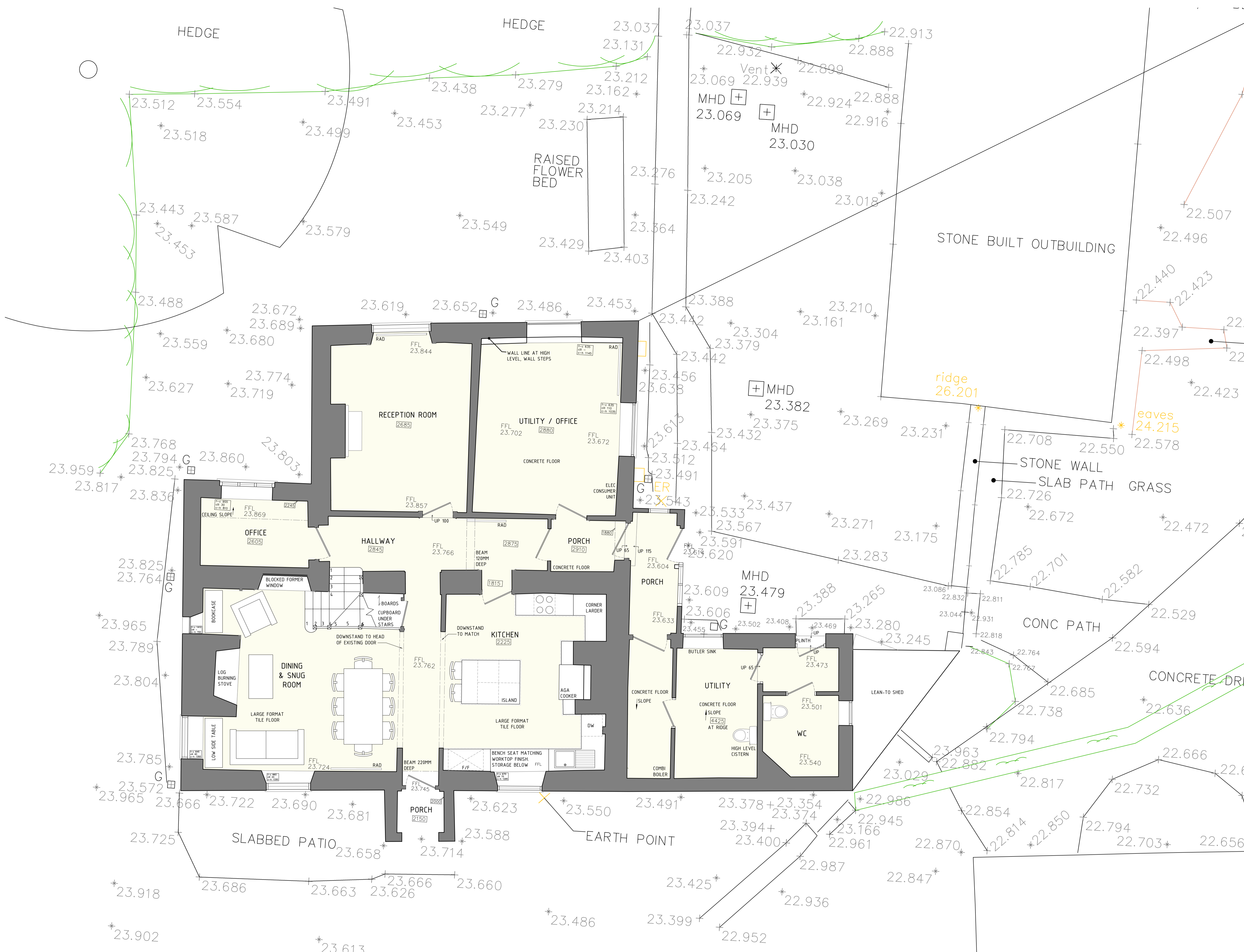
PROPOSED GROUND FLOOR PLAN 1:100 @ A3 // 1:50 @ A1 0 1 2 3 4 5 METRES
