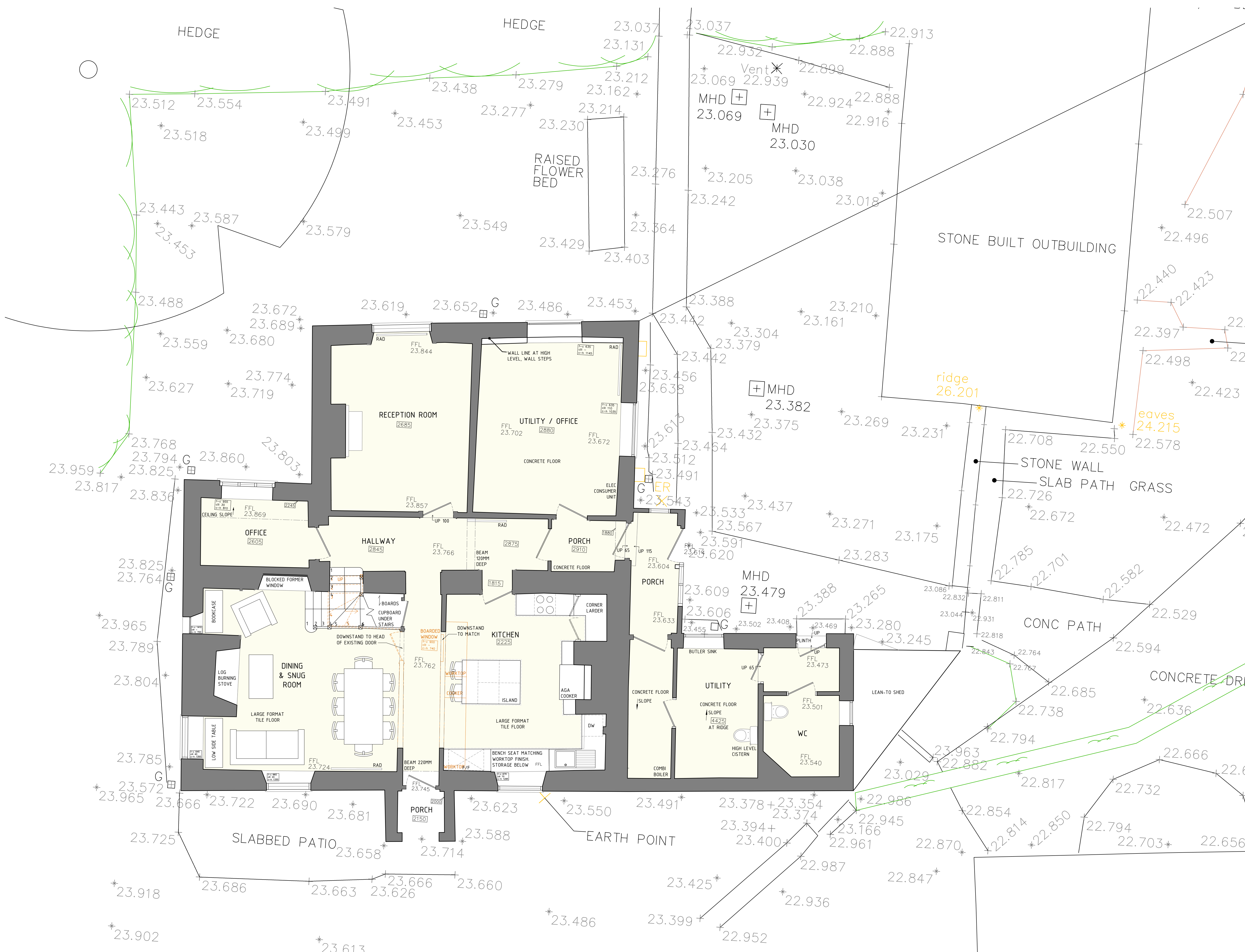
N PROPOSED GROUND FLOOR PLAN 1:100 @ A3 // 1:50 @ A1 0 1 2 3 4 5 METRES
