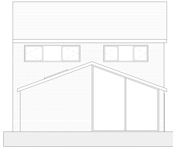
2 Rear Elevation 1 : 100
