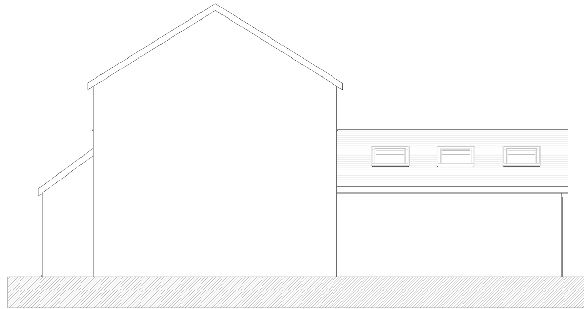
3 Side Elevation (East) 1 : 100
