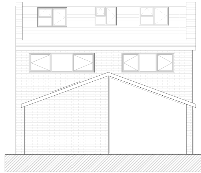
2 P- Rear Elevation 1 : 100
