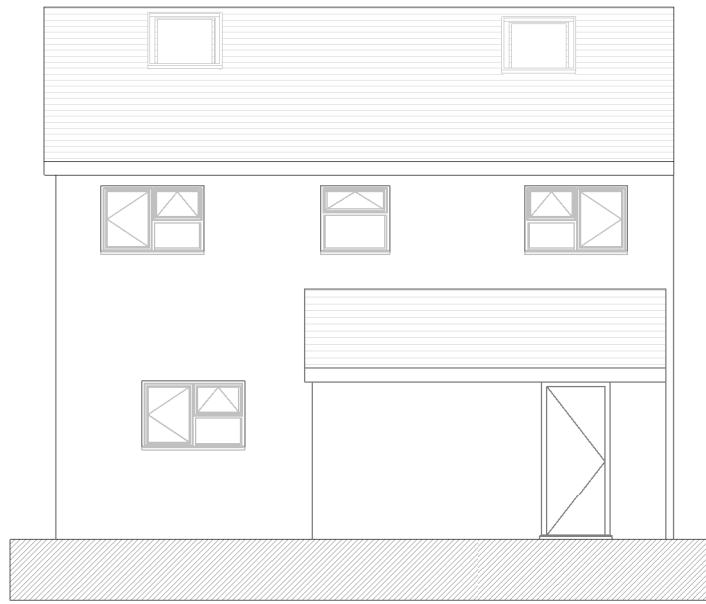
1 P- Front Elevation 1 : 100
