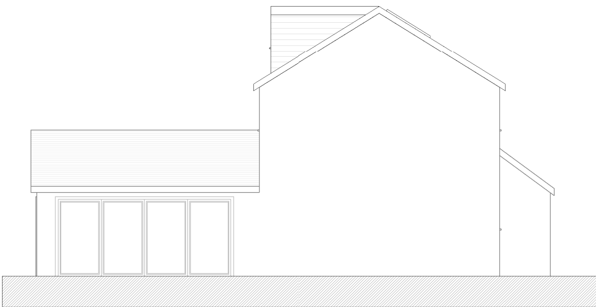
4 P- Side Elevation (West) 1 : 100
