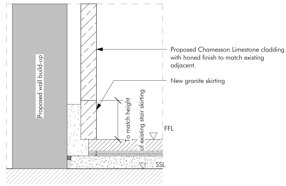
1 Basement Link - Chameson Cladding / Granite Skirting 1 : 5
