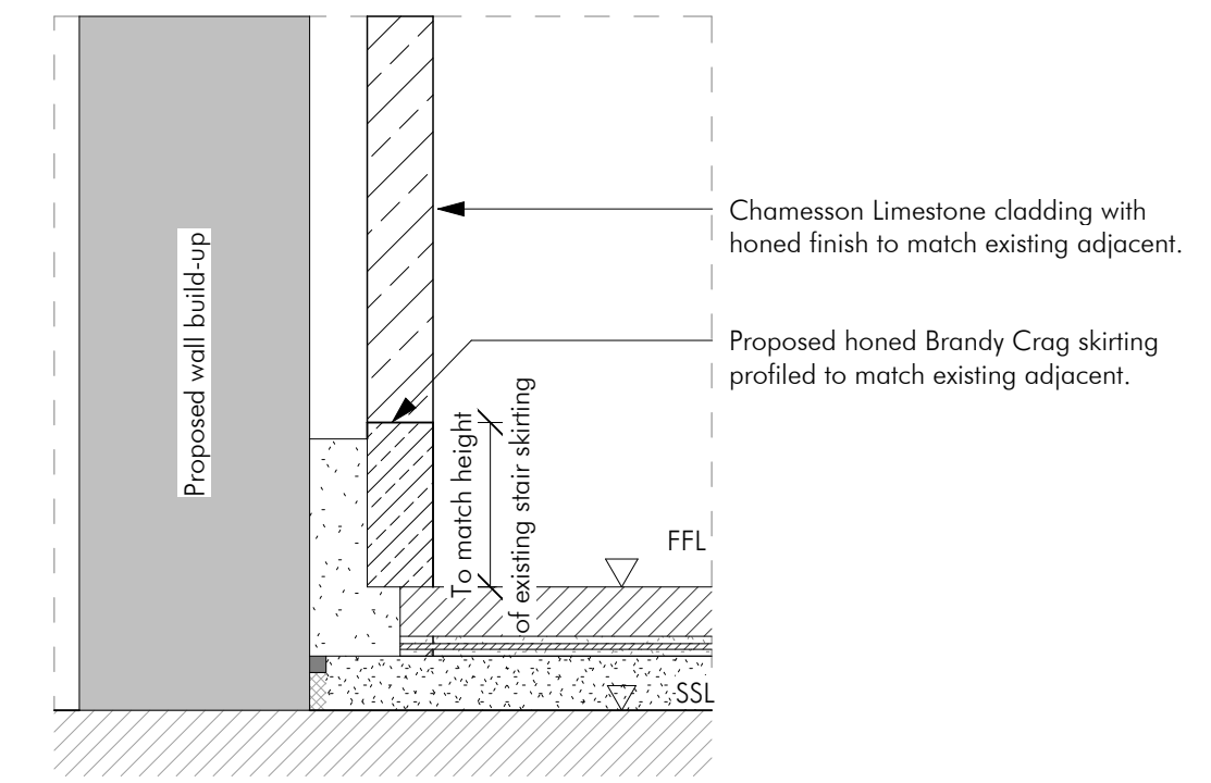
4 Basement - Link Landing / Opening Proposed Granite Skirting 1 : 5
