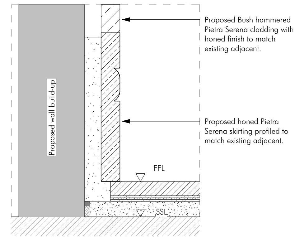
3 Basement - Column Skirting 1 : 5
