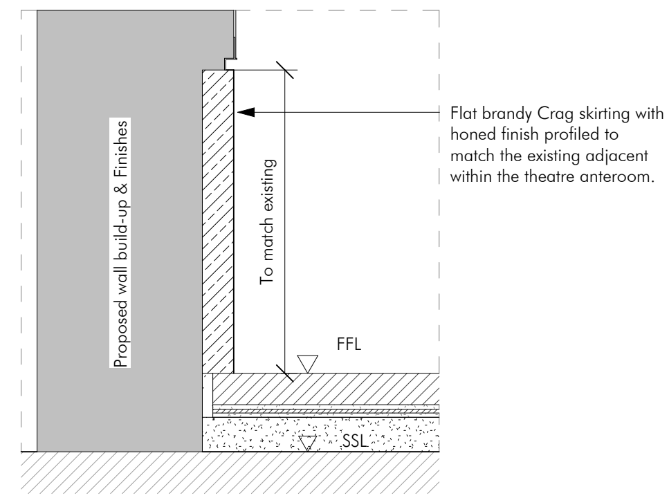
2 Basement - Painted Wall / Brandy Crag Skirting 1 : 5
