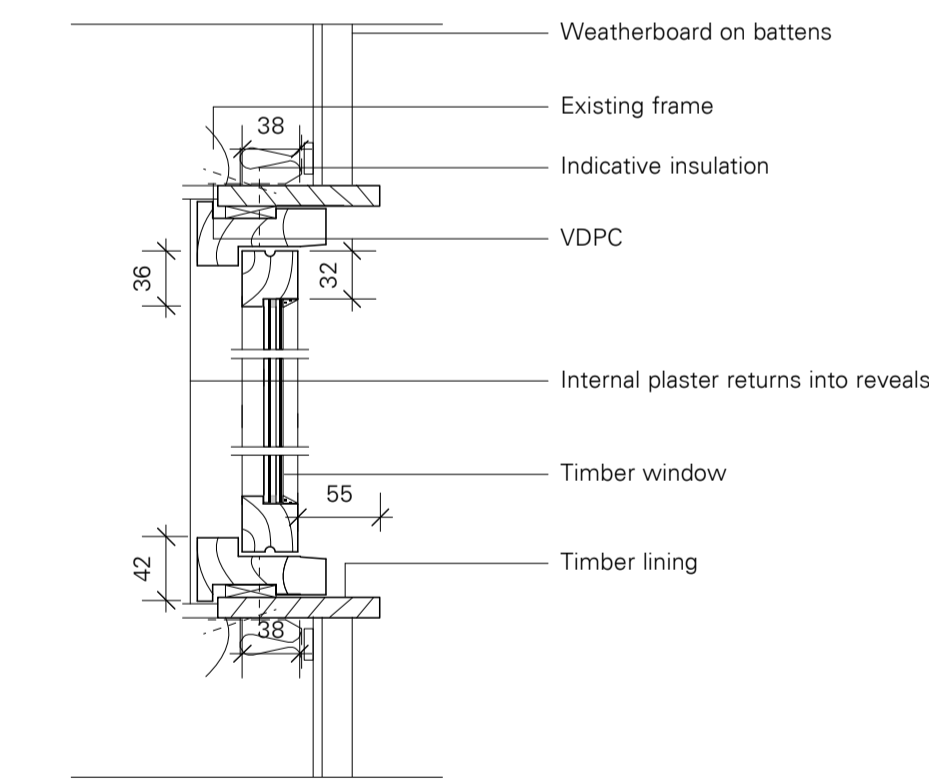
Typical Window Plan Detail 1:5
