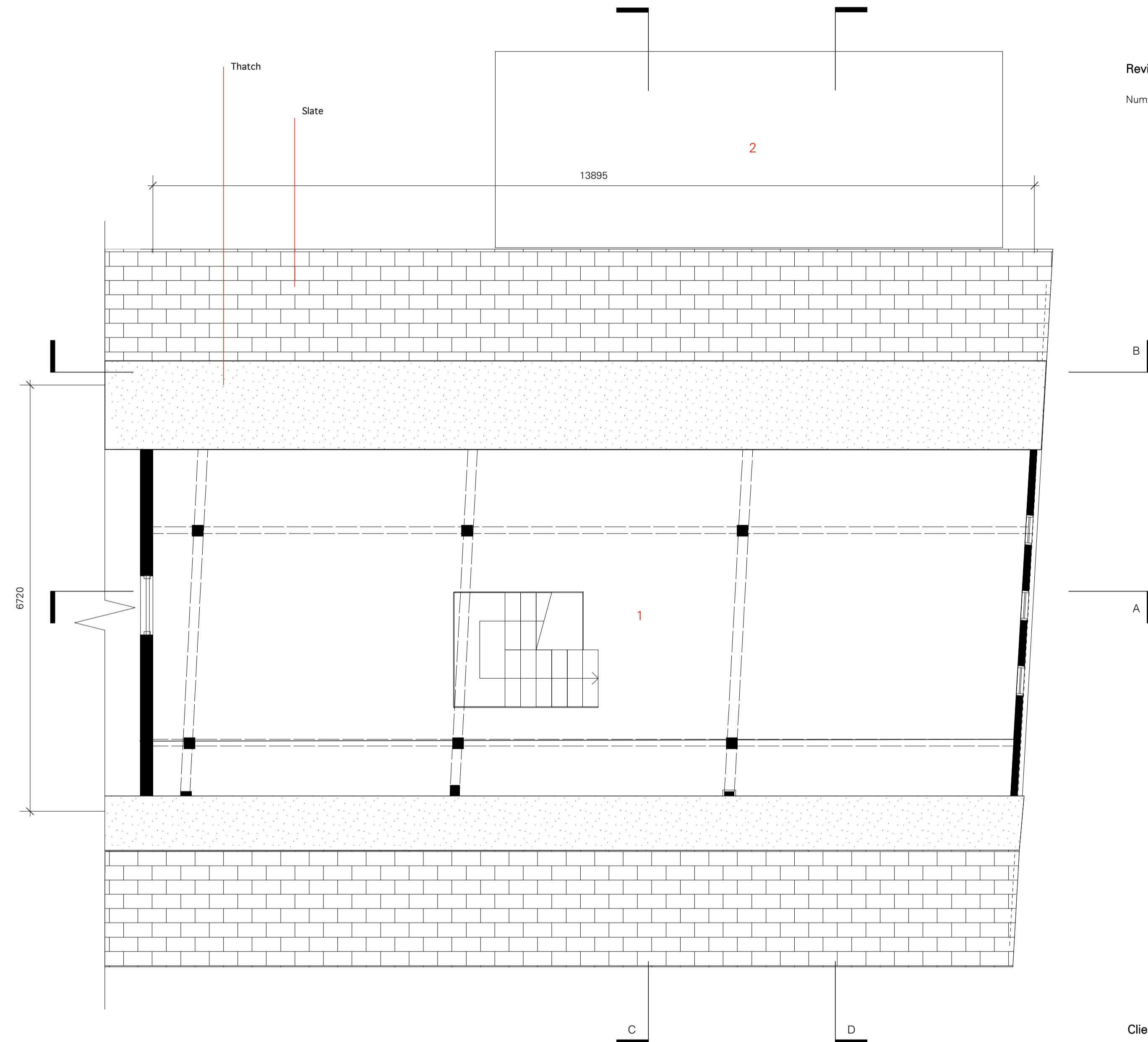
Proposed Loft Plan 1:50
