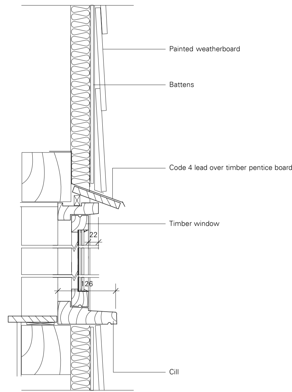
Typical Window Section Detail 1:5
