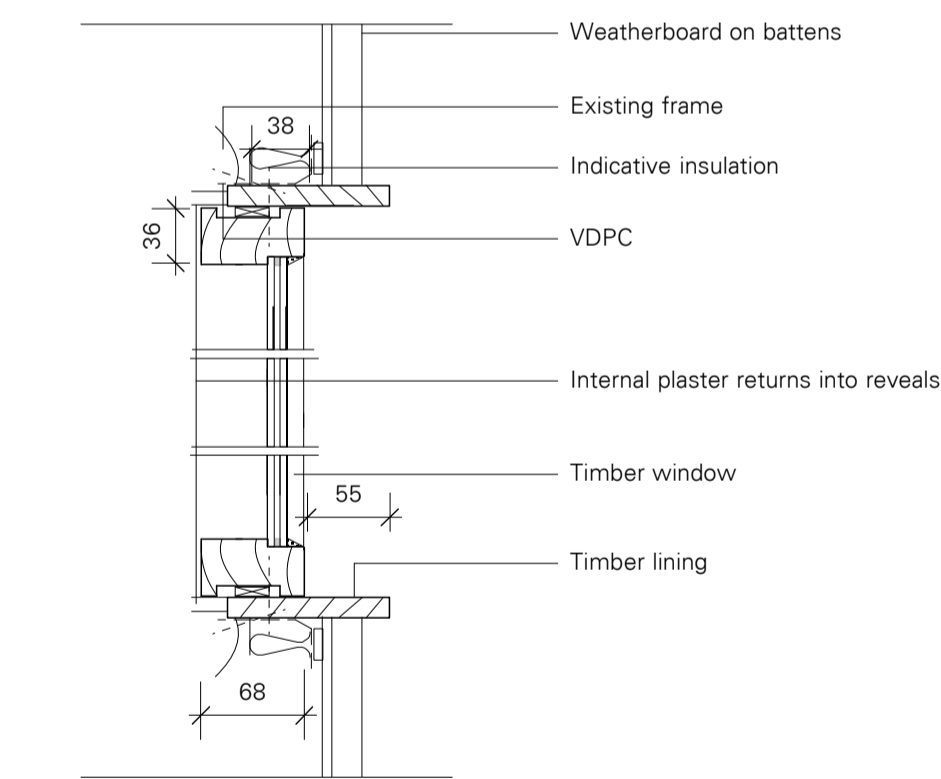
Typical Fixed Window Plan Detail 1:5
