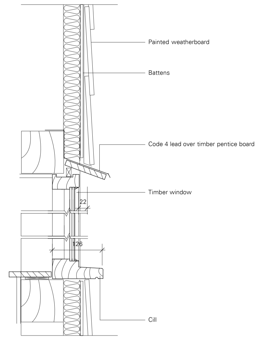
Typical Fixed Window Section Detail 1:5
