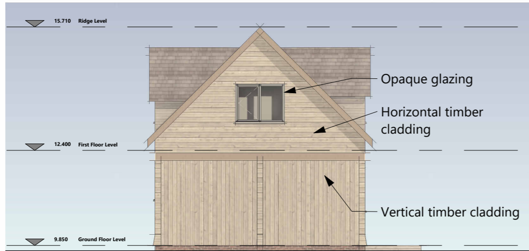
01 Front Elevation 1 : 100 @ A3
