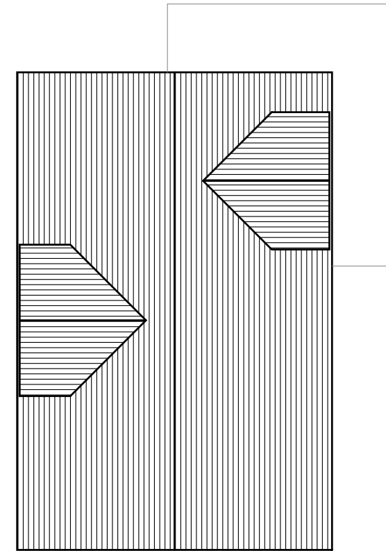
03 Proposed Roof Plan SCALE 1:100 @A3
