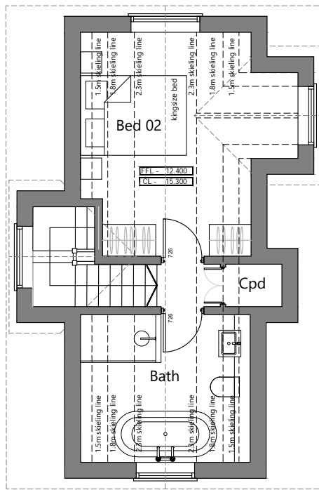
02 Proposed First Floor Plan SCALE 1:100 @A3
