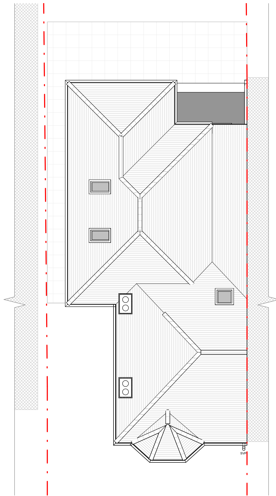
Roof Plan
