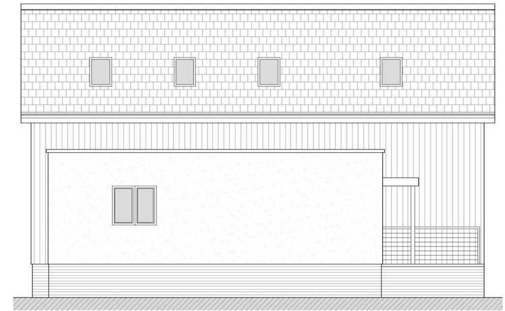
NORTH EASTERN ELEVATION
