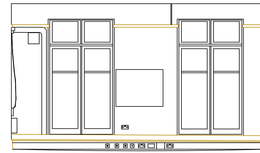
ROOM 4 ELEVATION ④ \Delta 67.00m
