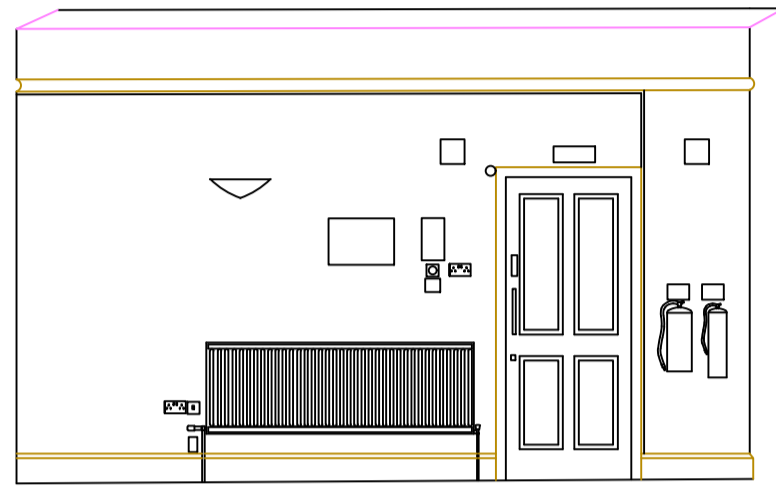
ROOM 4 ELEVATION ⑤ \Delta 67.00m
