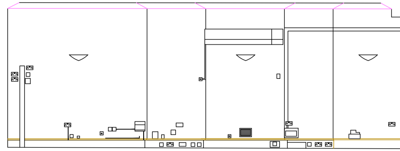
ROOM 4 ELEVATION ⑦ \Delta 67.00m
