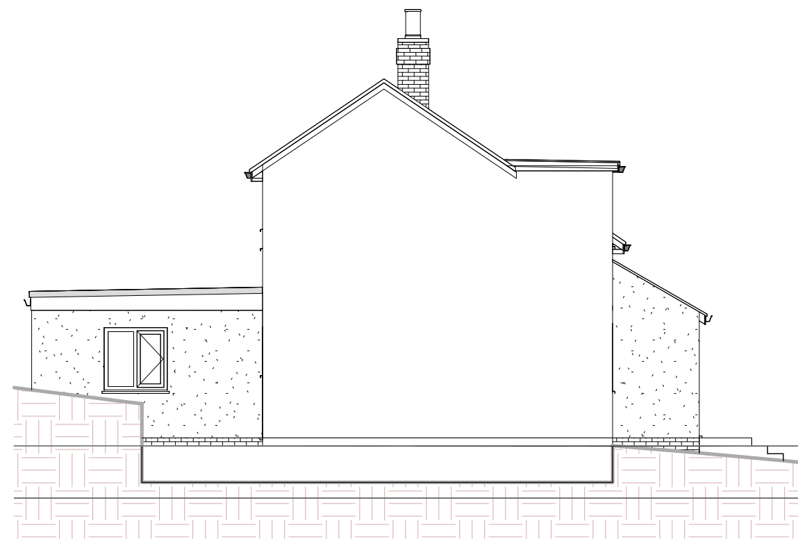
3 EP-304 Rev2 LEFT (PROPOSED) 1 : 100
