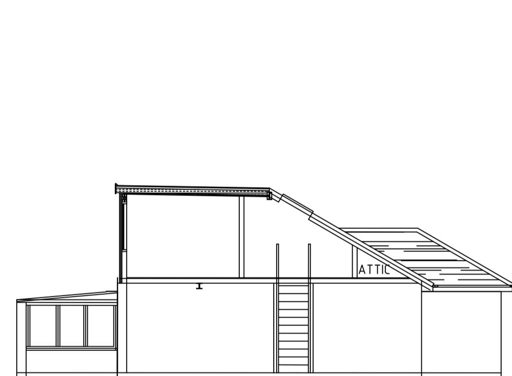
SECTIONAL SIDE ELEVATION
