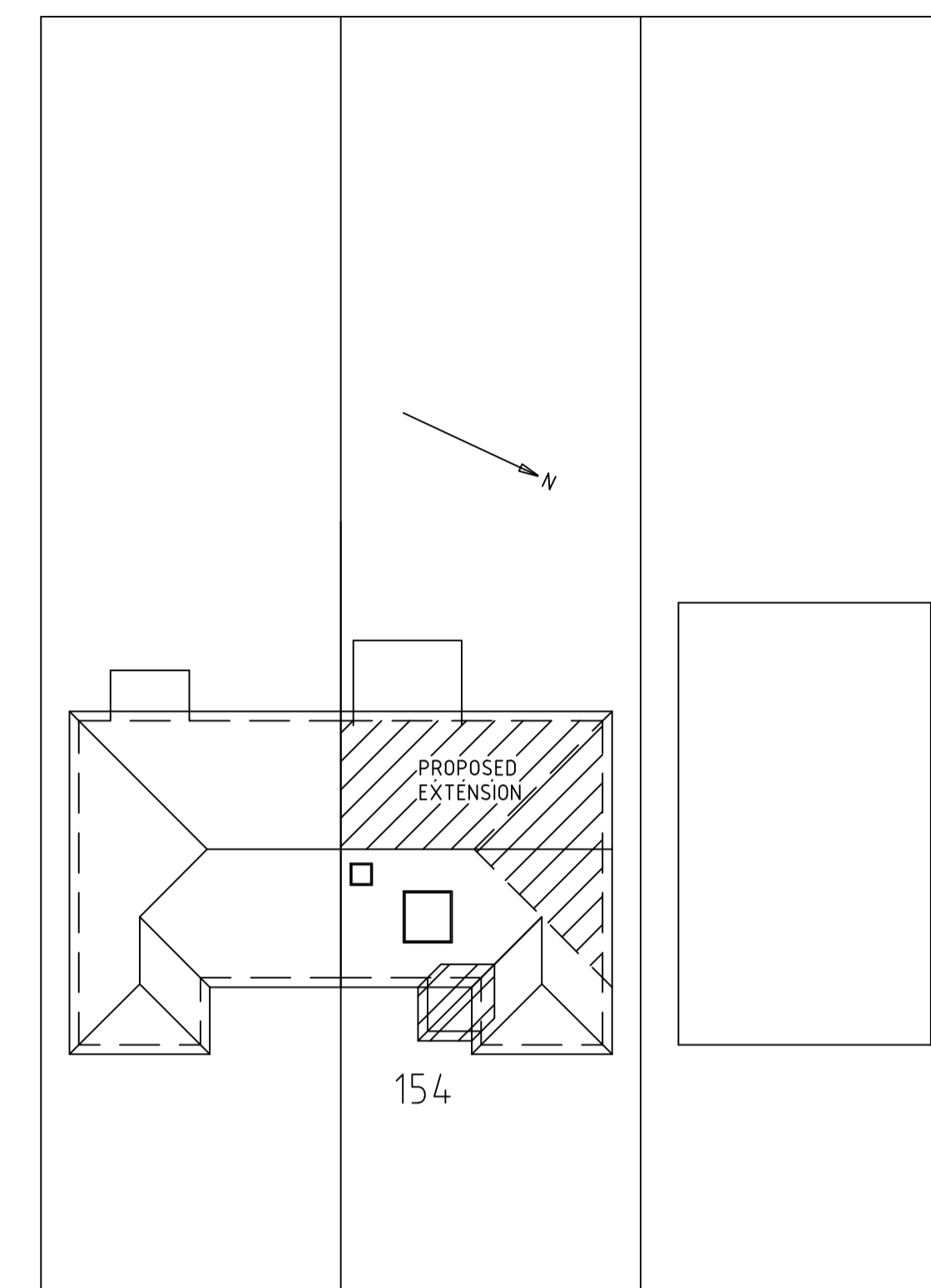
PROPOSED SITE/BLOCK PLAN SCALE: 1/200
