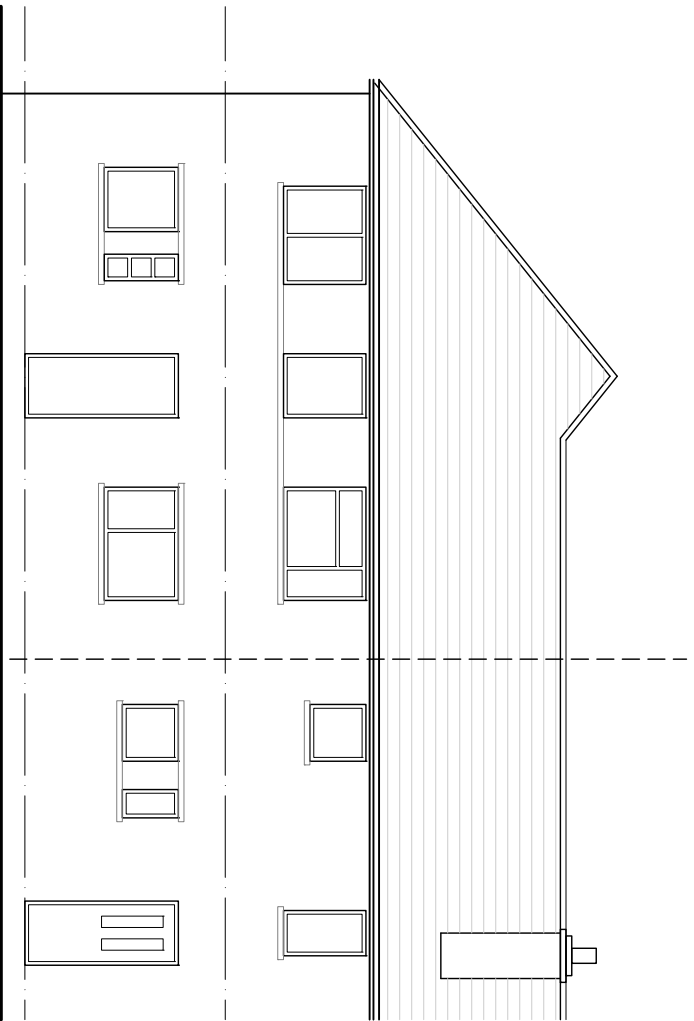
North West (Front) Elevation
