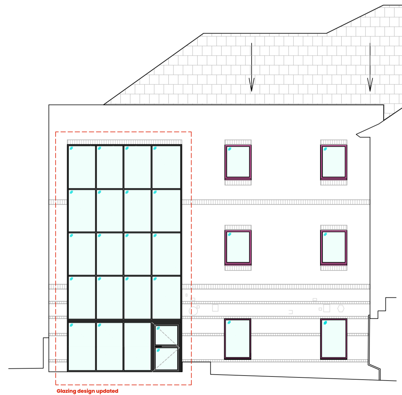
PROPOSED REAR ELEVATION B SCALE - 1:100
