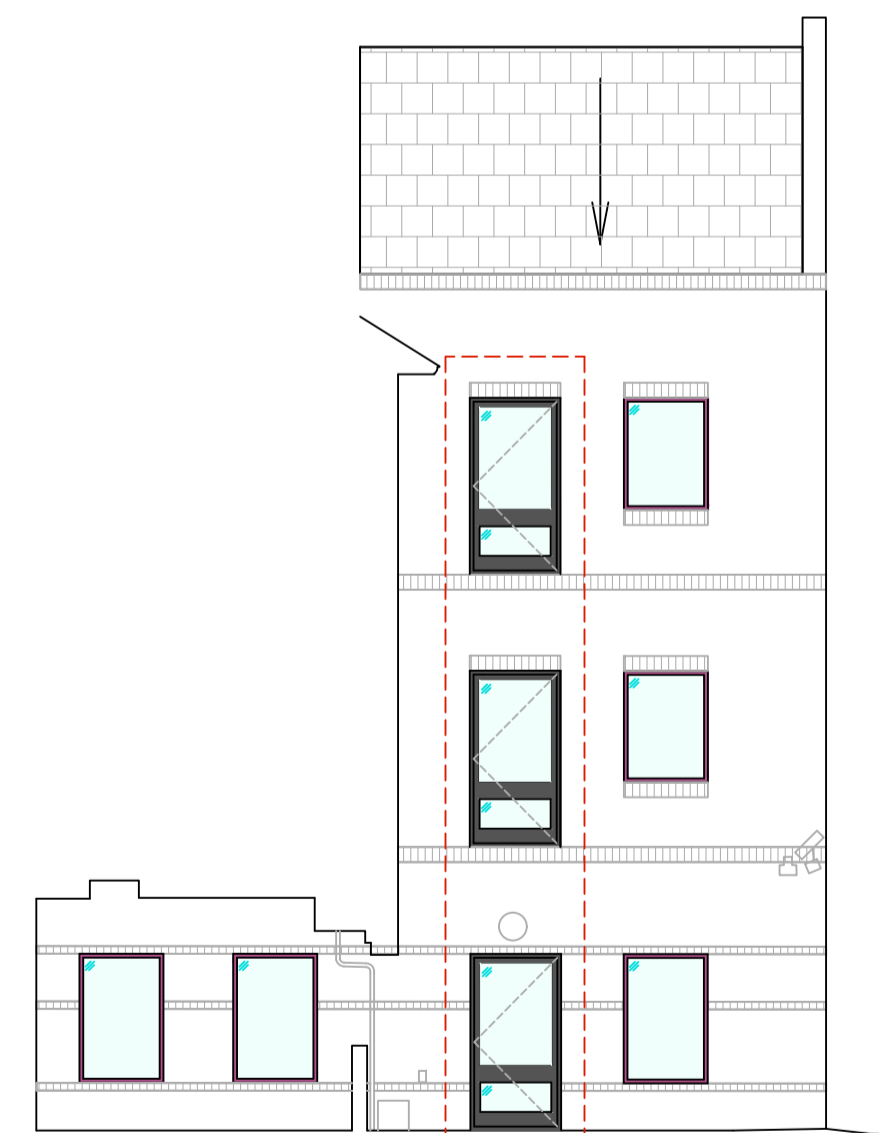
EXISTING REAR ELEVATION C SCALE - 1:100
