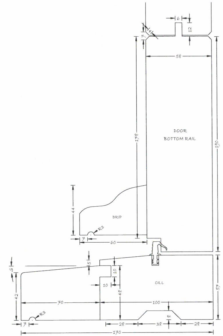
SECTION THROUGH CILL & BOTTOM DOOR RAIL
