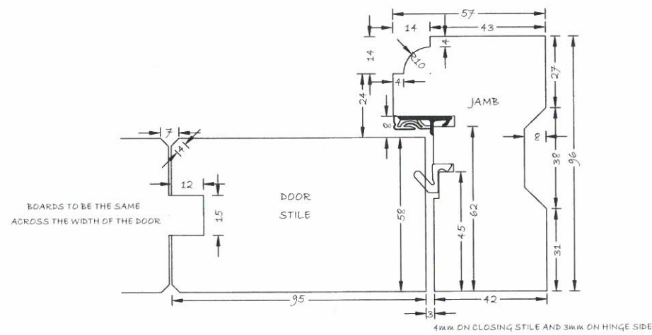
SECTION THROUGH JAMB & DOOR STILE
