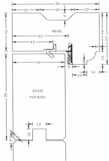
SECTION THROUGH HEAD & DOOR TOP RAIL
