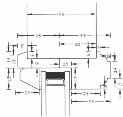
SECTION THROUGH TOP & SIDES OF VISION PANEL
