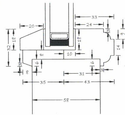
SECTION THROUGH BOTTOM OF VISION PANEL
