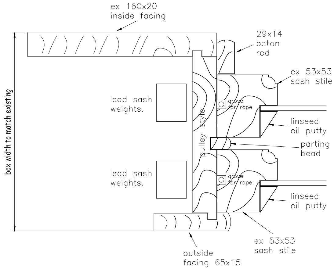
SIDE SECTION THRU' CASE
