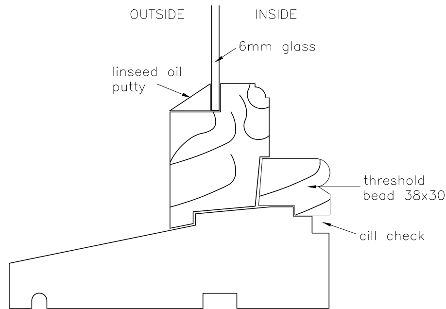
CILL DETAIL
