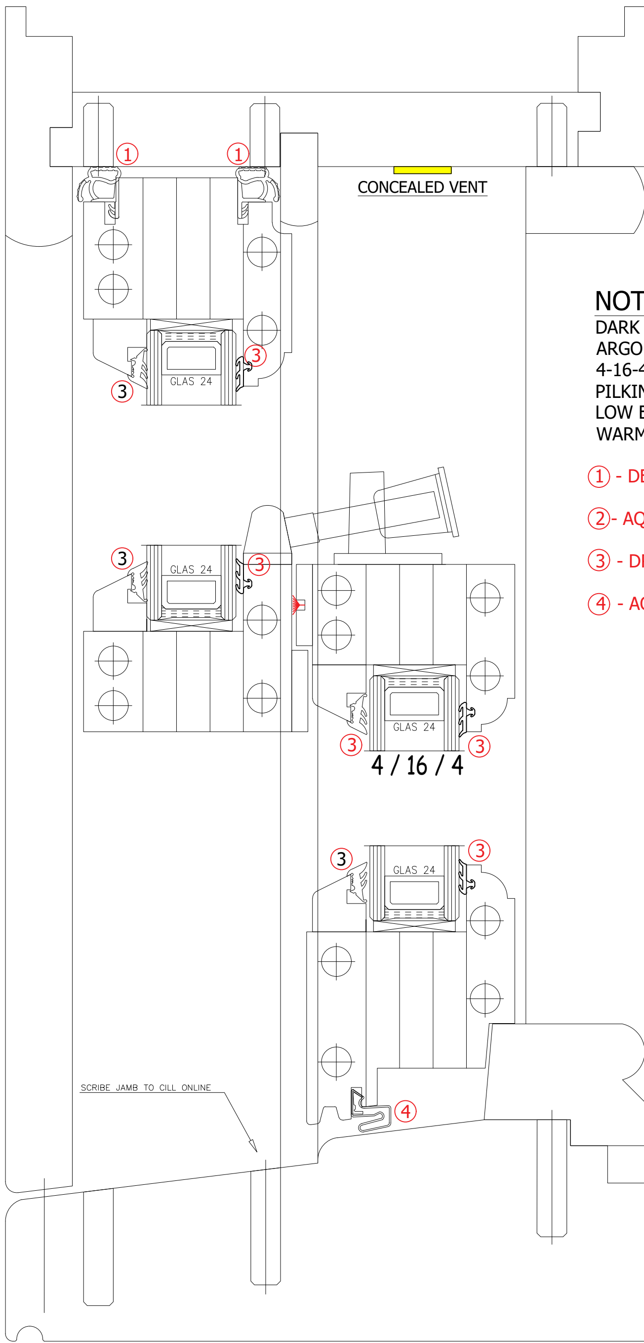
PROPOSED SASH & CASE WINDOW SECTION SCALE : 1.1
