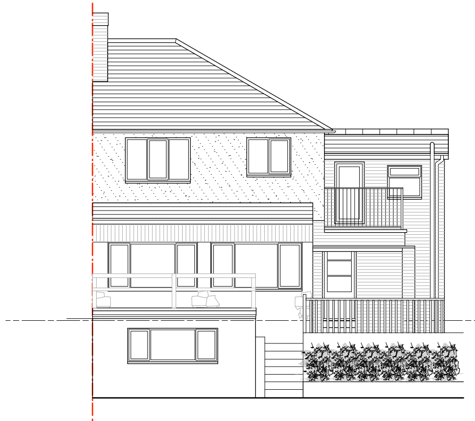
REAR (NORTH WEST) ELEVATION
