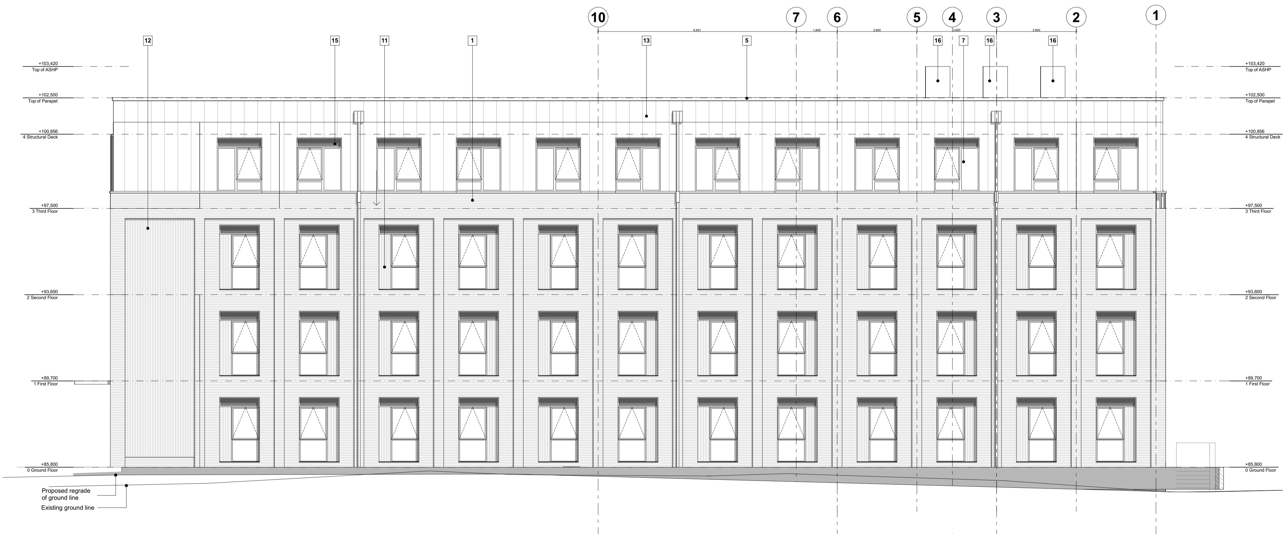
E04 Eastern Elevation
