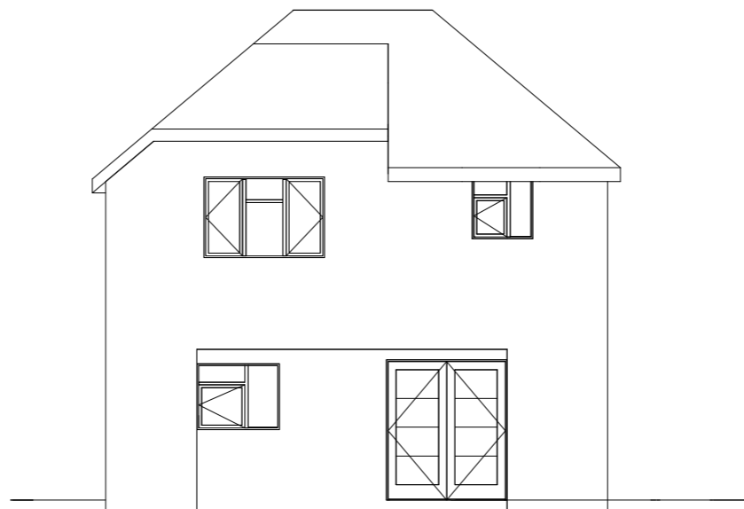
2 Existing South Elevation 1 : 100
