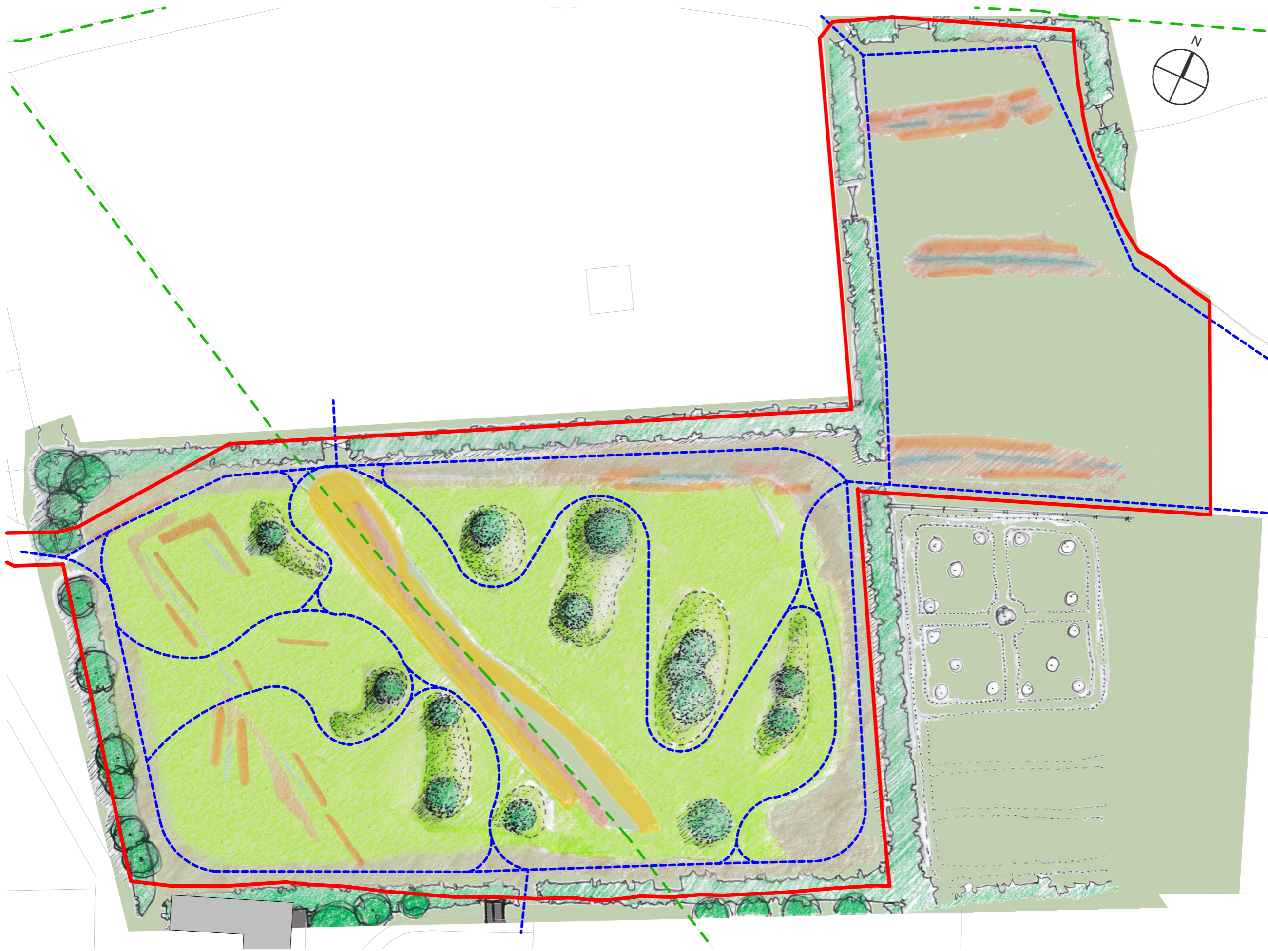
SKETCH PLAN - DETAIL 1:500
