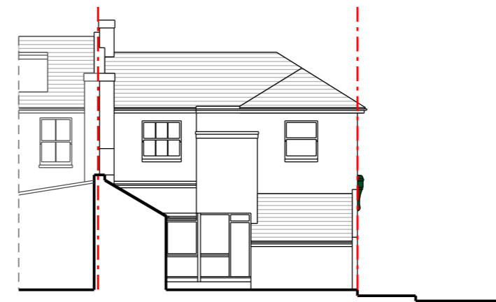
Rear Elevation (North)
