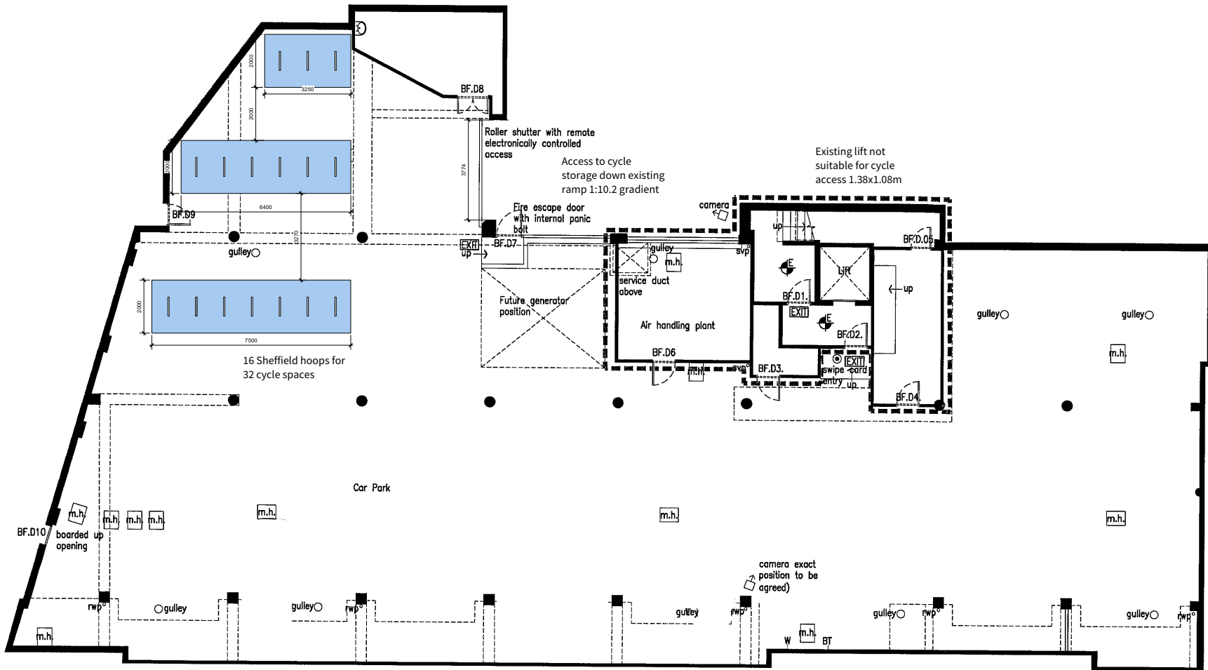
Proposed Bike Storage To Basement 1: 200 @ A3
